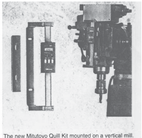
The new Mitutoyo Quill Kit mounted on a vertical mill.
